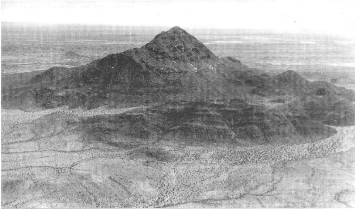
Plate 1: Aerial view of the Okenyenya igneous complex showing Johannes Berg in the foreground with arcuate gabbro and syenite ridges and Okenyenya Berg in the background, with the Adams Shoulder alkaline gabbros on the left. The central oligoclase essexite intrusion forming the summit of Okenyenya Berg is clearly visible, as is the surrounding nepheline syenite ring seen between the essexite and Adams Shoulder.
