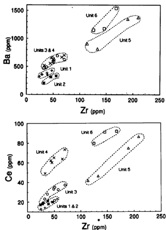
Figure 2: Variation of selected incompatible trace elements in samples collected from a transect across the tholeiitic gabbro - quartz monzodiorite body, showing the compositional differences between 6 intrusive units. Samples within each compositional unit were generally, but not exclusively, from adjacent neighbouring sampling sites along the traverse, and can thus be related to individual magmatic injections. Unit numbers increase towards the outer contact of the complex.
