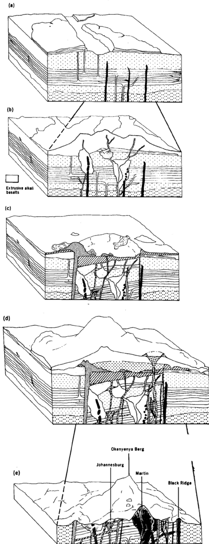
Figure 3: Simplified sketch block diagrams showing the evolutionary model proposed for Okenyenya igneous complex. The front faces of the blocks represent generalised sections through the centre of the complex in an approximately NW-SE direction. Since no volcanic rocks are preserved at Okenyenya, the extrusive features are necessarily speculative but are included to give some perspective to the intrusive structures. No accurate scale is implied by the diagrams which do not attempt to portray accurately the extent of surface denudation occurring during the 5 million years of development of the igneous complex. Individual block diagrams represent the stages of emplacement described in the text: a, emplacement of near flat-lying tholeiitic gabbro sheets; b, emplacement of high level magma chambers of alkaline gabbro; c, cauldron subsidence of the complex coincident with the injection of syenite and quartz-syenite magmas as a major peripheral ring dyke and a series of smaller arcuate dykes and sills. For simplicity, the tholeiitic gabbros are shown to dip uniformly to the west; d, emplacement of the Okenyenya Berg nepheline syenite/essexite intrusions on the northern margin of the former complex, flexuring of the central "plate" within the ring fault, and injection of highly alkaline magmas as dykes, plugs and pipes into the fractures thus produced; e, present day Okenyenya igneous complex. Ornamentation is the same as in Fig. 1.
